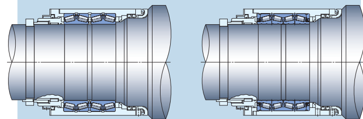
(1) Open type four-row tapered roller bearing
